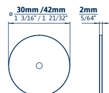
Knopf | knob: 2464-33PB12 Unterlagsplatte | base plate: 2490-42PB12
